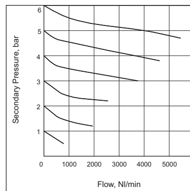
1/2" REGULATOR
