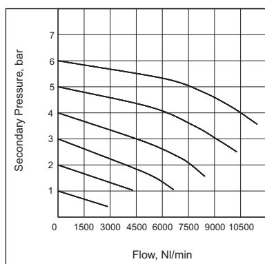
3/4" REGULATOR
