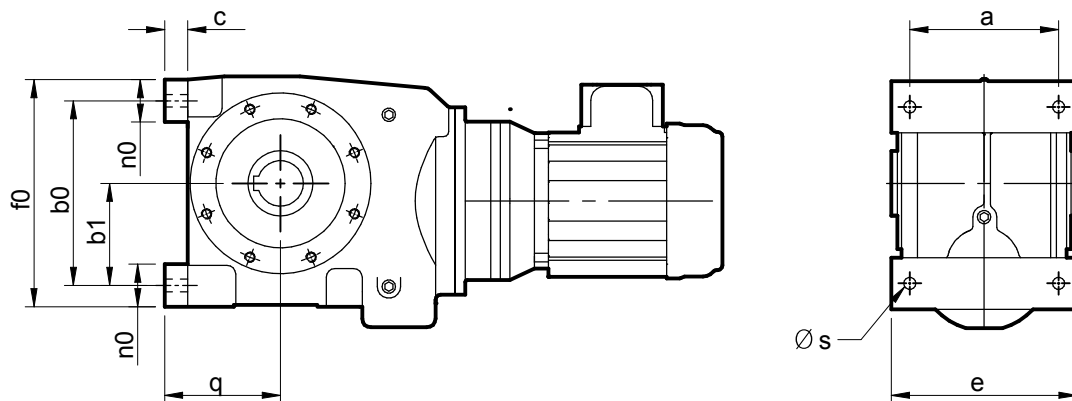
STANDARD UNIT WITH END MOUNTED FEET
