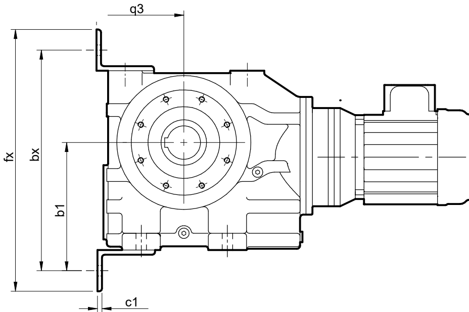
STANDARD UNIT WITH END MOUNTED FEET
