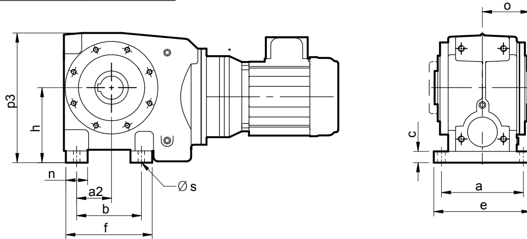
STANDARD UNIT WITH BASE MOUNTED FEET
