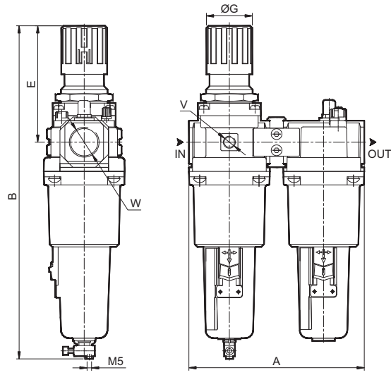
Model FRCLM17...-MM/S
