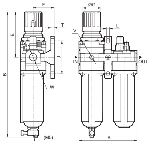
Model FRCLM17...-MM/W
