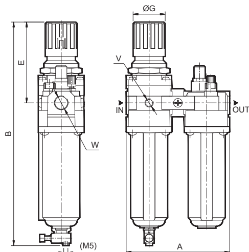
Model FRCLM17...-MM/S
