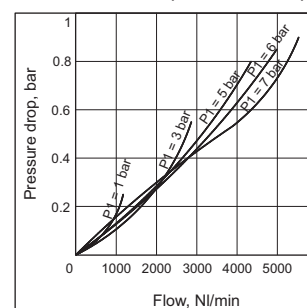
1/2 FILTER (0.1 micron)
