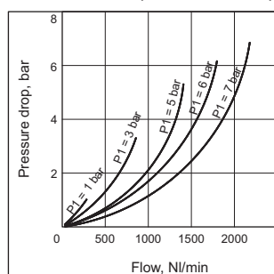
1/4 FILTER (0.01 micron)
