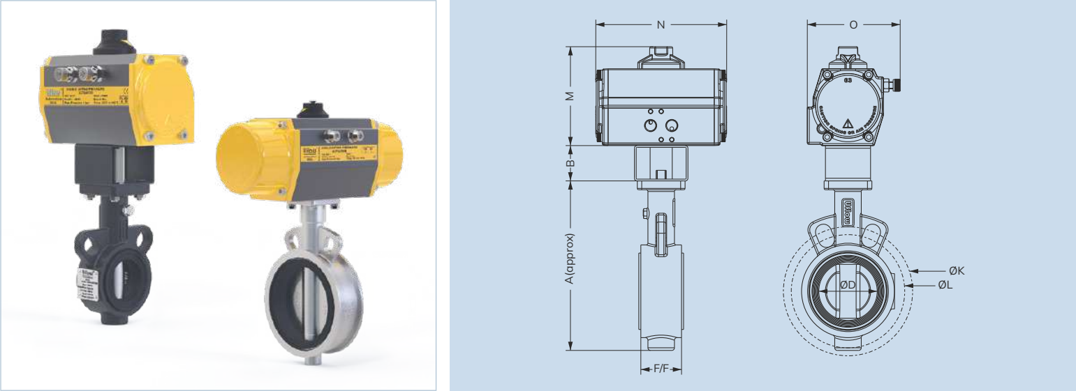
Technical Data - Butterfly Valve with Double Acting Actuator (All dimensions are in mm) All dimensions are approx.
