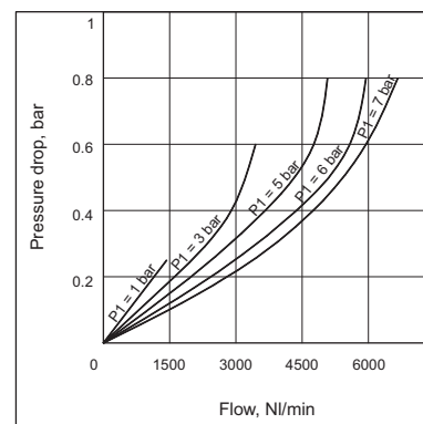
1/2" LUBRICATOR
