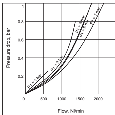
1/4" LUBRICATOR
