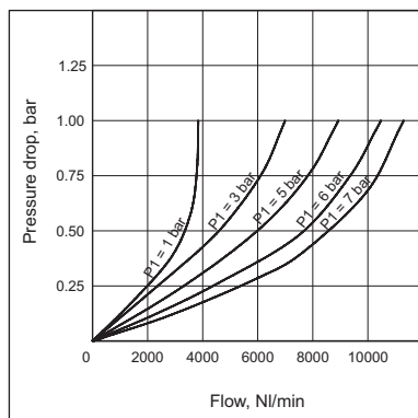
3/4" LUBRICATOR
