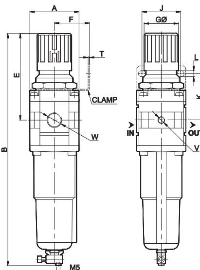
Model FRC15...-MM (Without level indicator)
