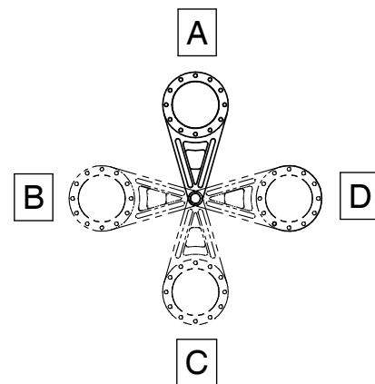
MOUNTING POSITIONS
